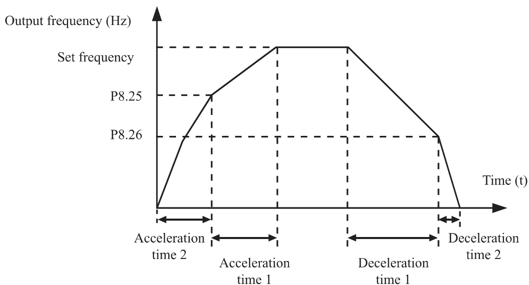
Figure 4-17 Acceleration/deceleration time switchover
