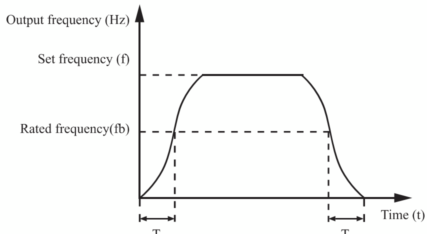
Figure 4-1 S-curve acceleration/deceleration B
