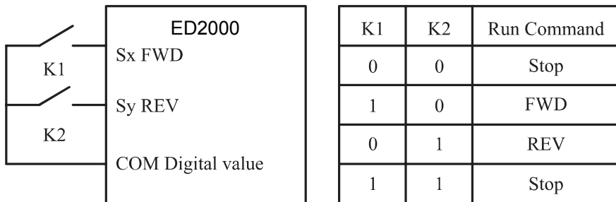
Figure 4-8 Setting of two-line mode 1
