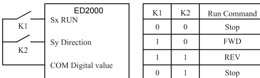
Figure 4-9 Setting of two-line mode 1
