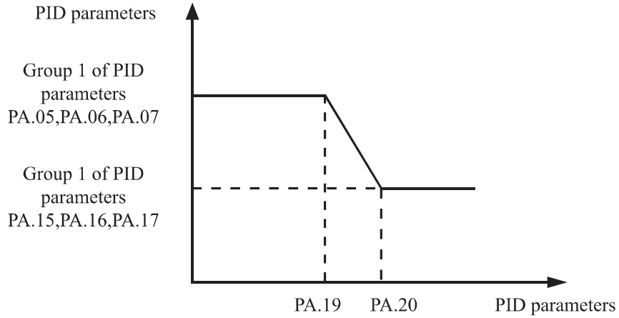
Figure 4-24 PID parameters switchover
