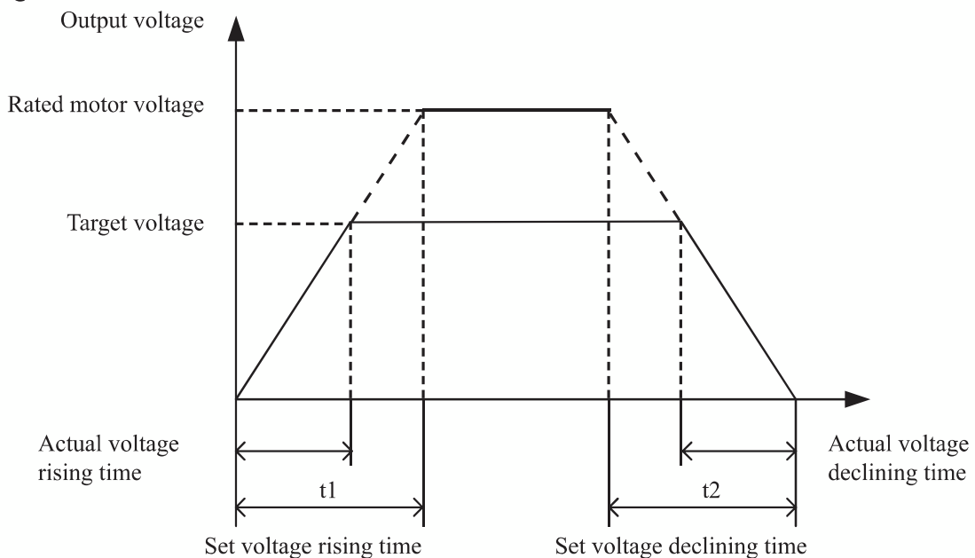
Figure 4-7 Voltage of V/F separation
