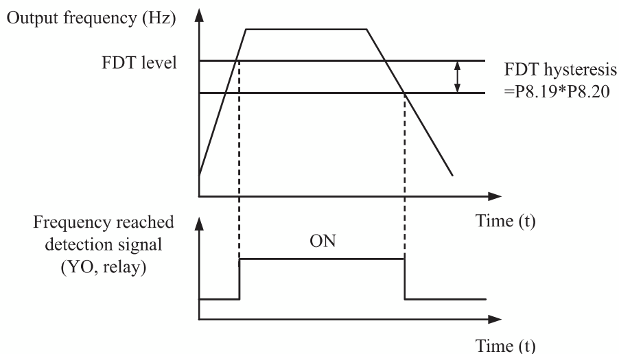
Figure 4-14 FDT level
